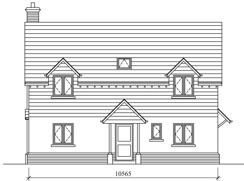
NORTH ELEVATION
