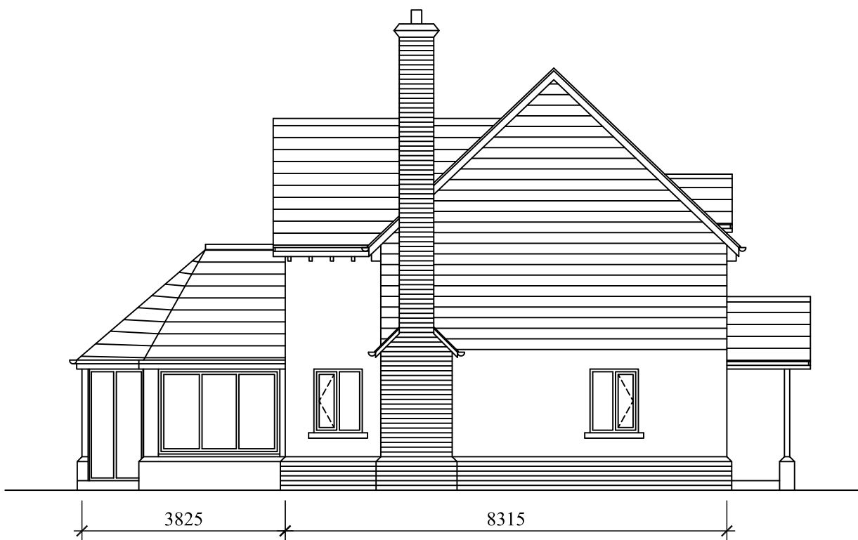
WEST ELEVATION
